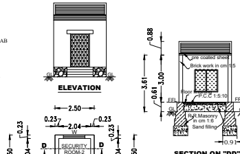
SECTION ON "DD"
