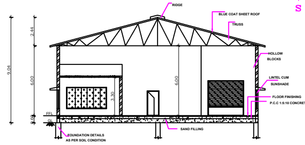
SECTION ON "B-B"
