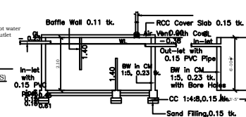
SECTION - SEPTIC TANK & SOAK PIT
