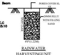
RAINWATER HARVESTING UNIT
