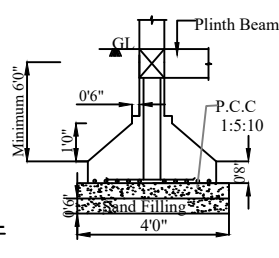
COLUMN DETAIL
