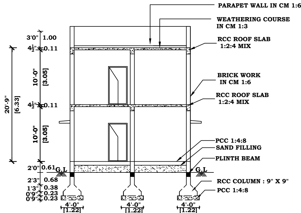
SECTION - KK
