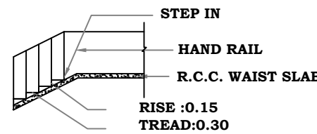
STAIR DETAILS
