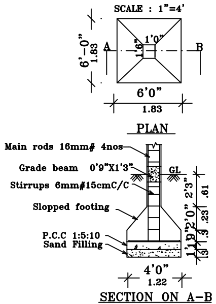
COLUMN DETAILS
