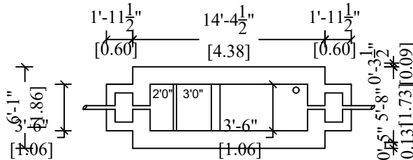
SEPTIC TANK DETAILS
