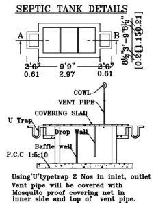
SEPTIC TANK DETAILS
