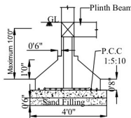
COLUMN DETAIL SCALE 1 : 50
