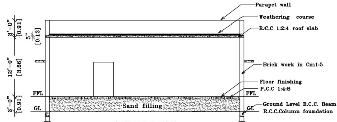
SECTION ON 'SK'
