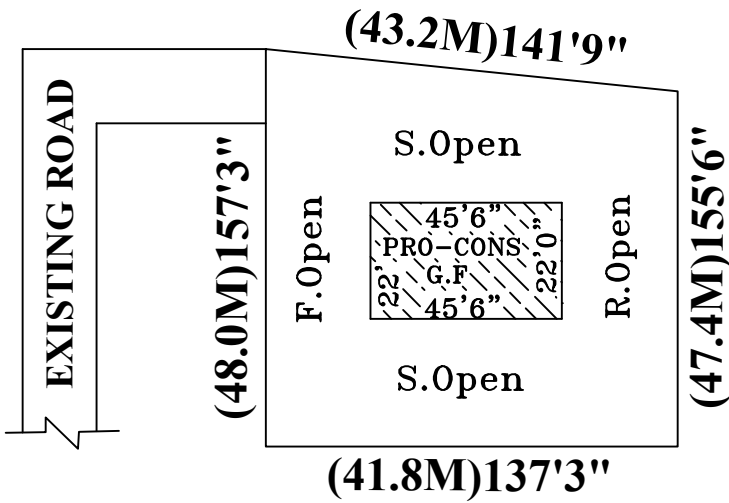
SITE PLAN
