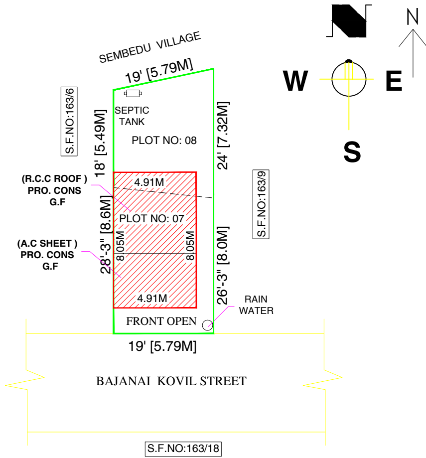
SITE PLAN
