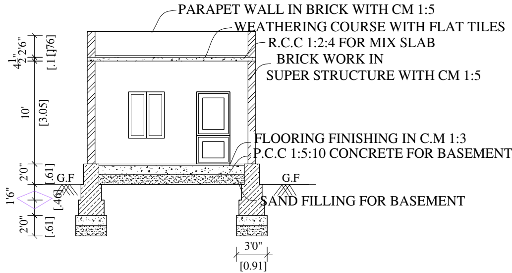
SECTION NO R-S
