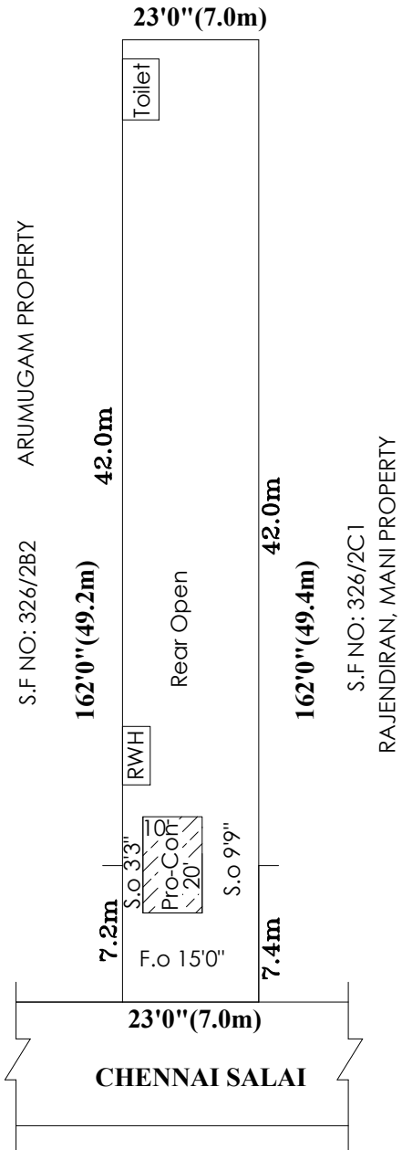
SITE PLAN
