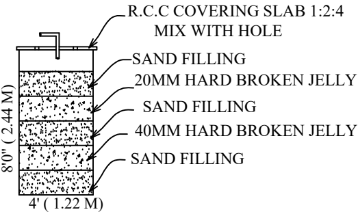
Section - Septic tank & Soak pit
