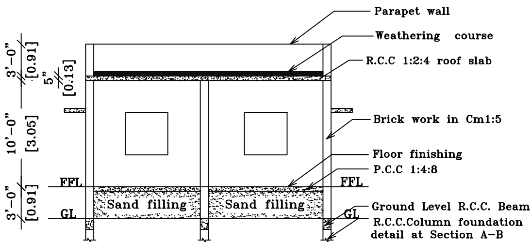
SECTION ON 'SA'
