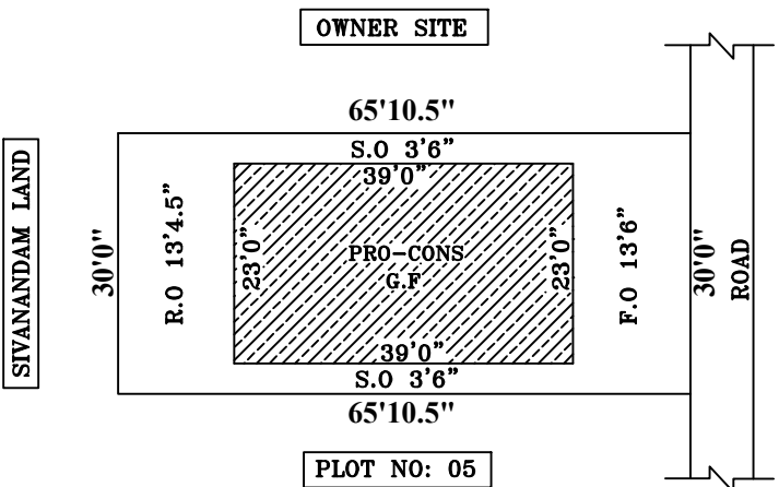
SITE PLAN
