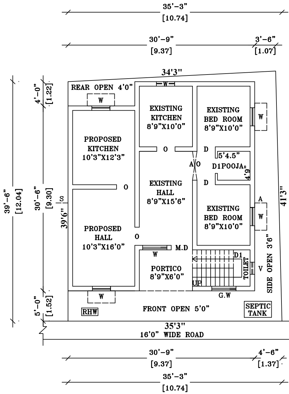
EXISTING GROUND & PROPOSED ADDITIONAL- CONSTRUCTION GROUND FLOOR PLAN
