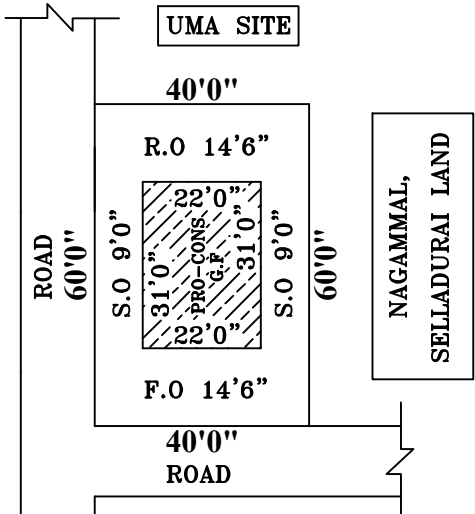
SITE PLAN SCALE: 1INCH=33FEET
