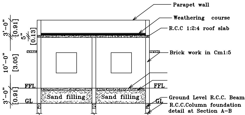
SECTION ON 'SA'
