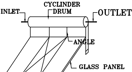
SOLAR ENERGY (NOT TO SCALE)
