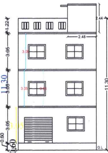
FRONT EVLAATION
