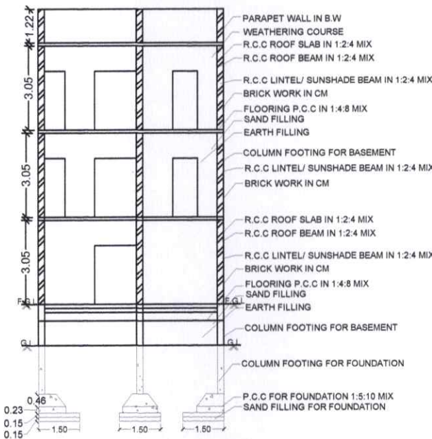
SECTION X-X
