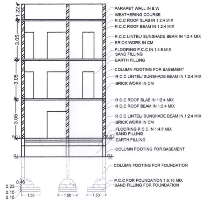
SECTION 'X'-X'
