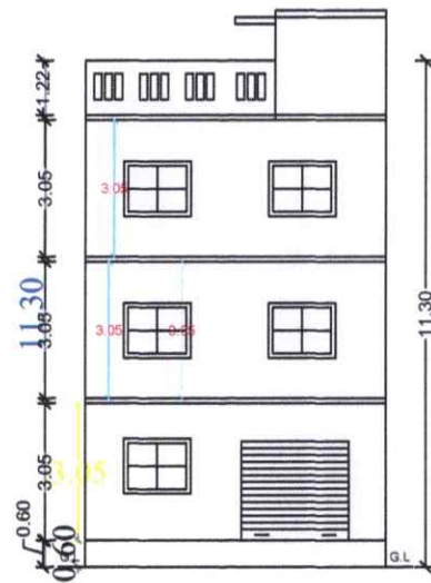
FRONT EVLAATION
