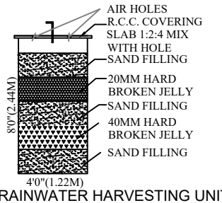
RAINWATER HARVESTING UNIT
