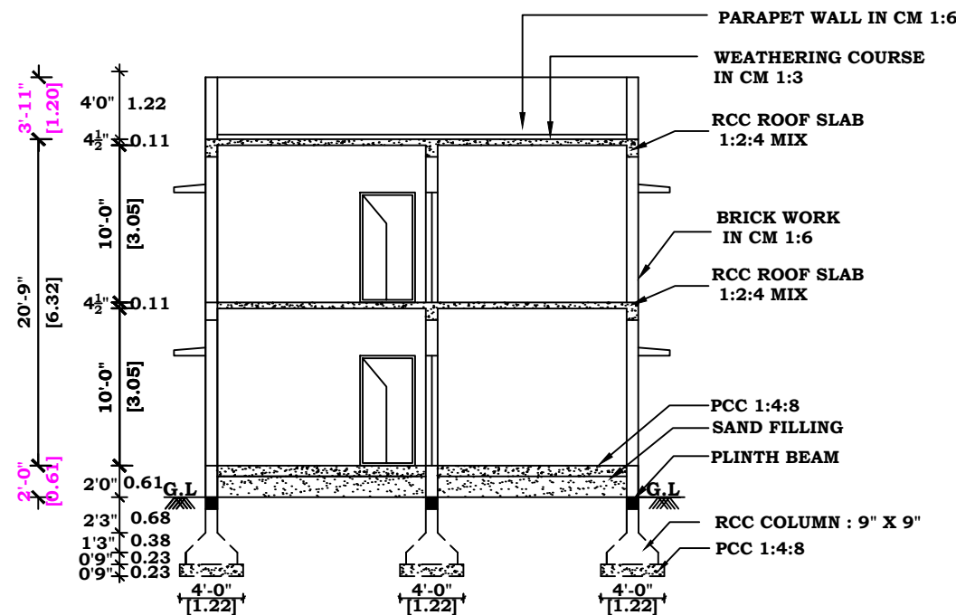
SECTION - KK
