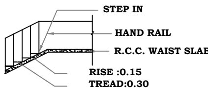
STAIR DETAILS
