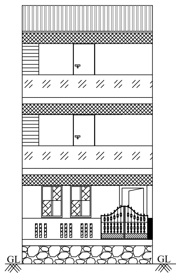
FRONT ELEVATION
