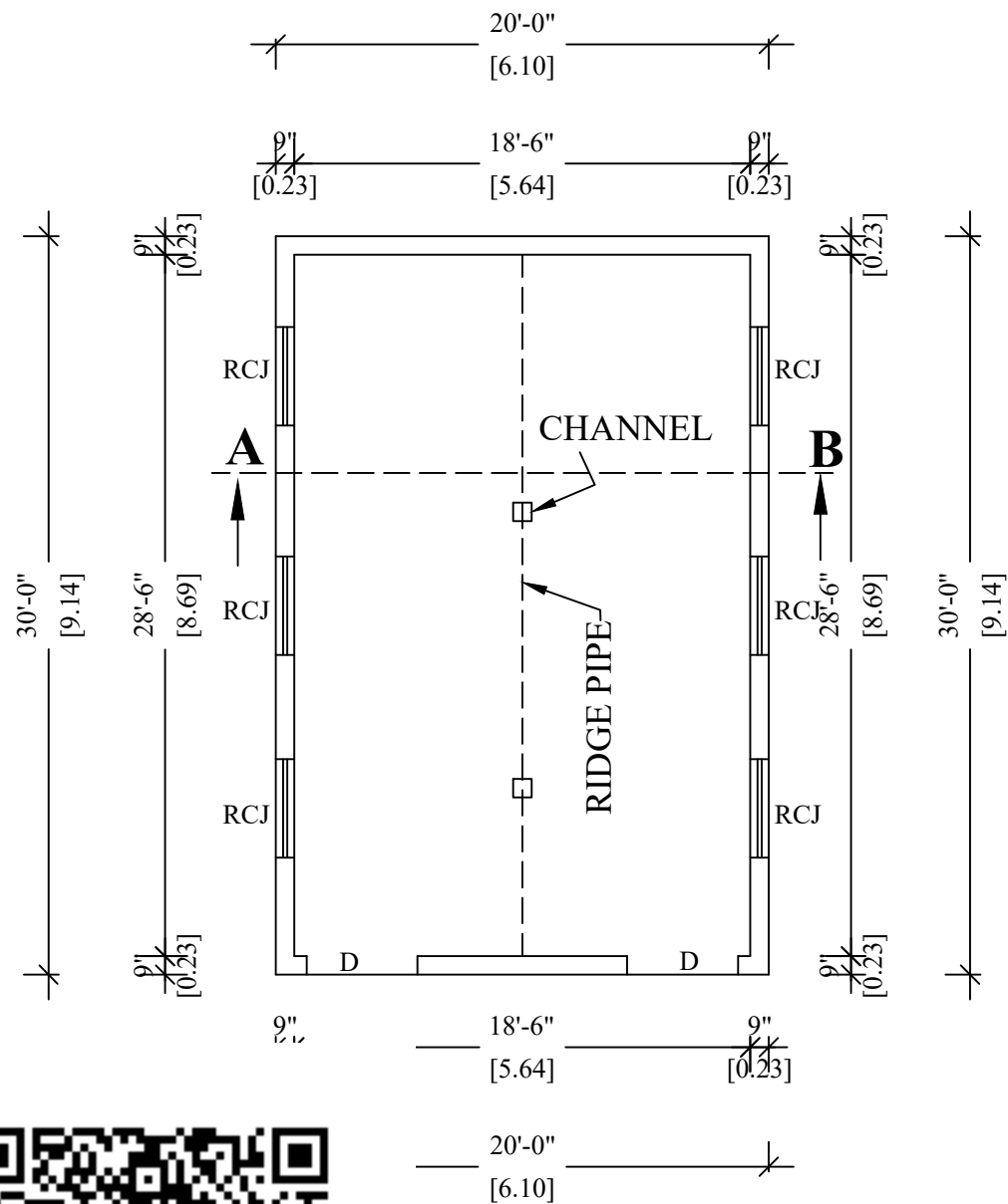
D FLOOR PLAN
