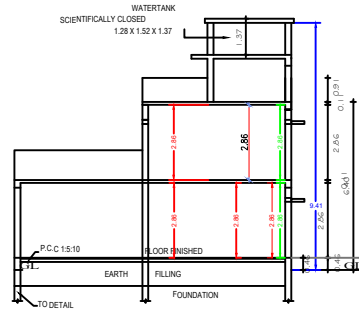
SECTION "A-B"
