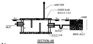
SECTION-AB
