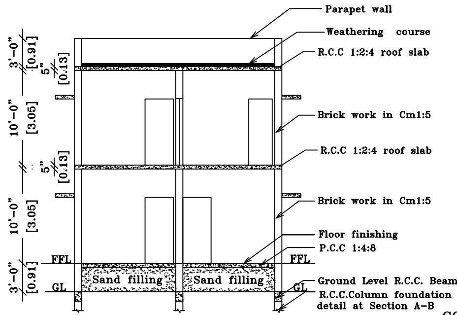
SECTION ON 'SK'
