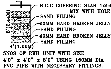
RAIN WATER HARVEST UNIT
