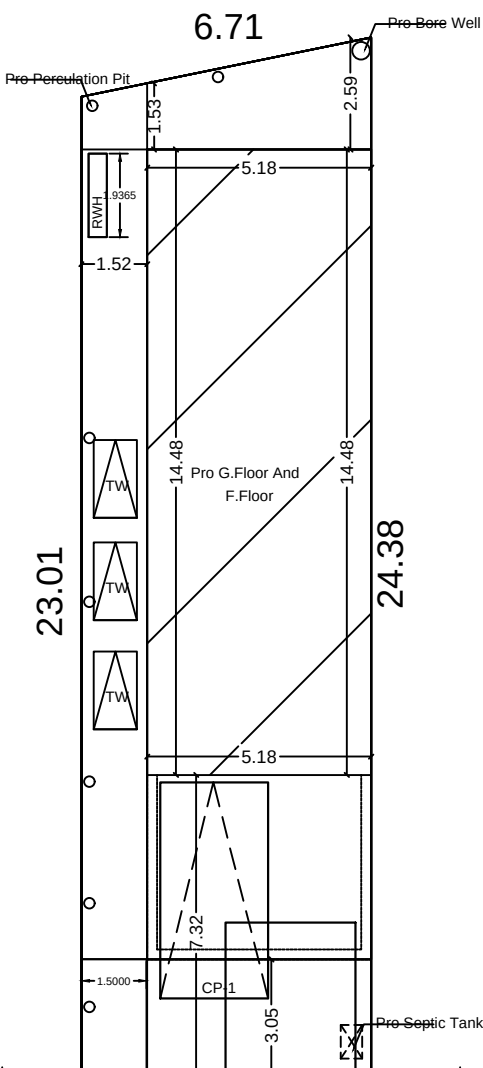
Exg 40'0" WIDE ROAD
