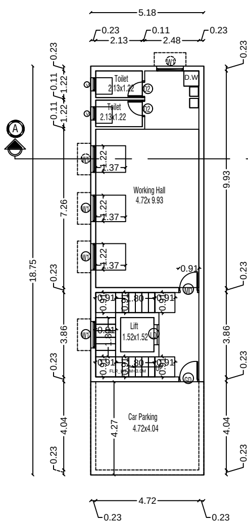
Pro Ground Floor Plan
