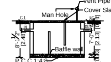
Section on BB'
