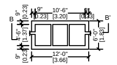
Plan Septic Tank Details
