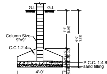
Column foundation Details
