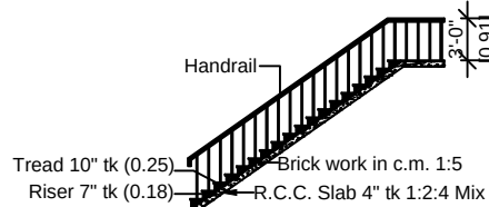
Staircase Details
