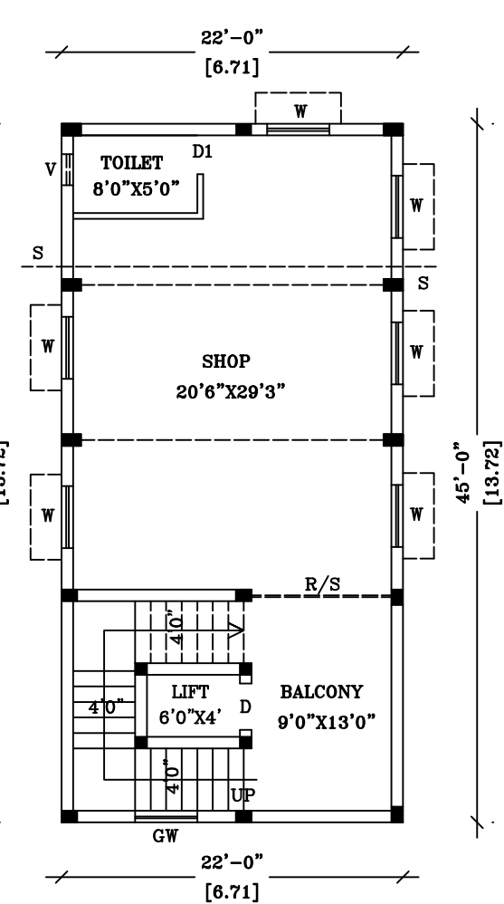
PROPOSED ADDITIONAL CONSTRUCTION FIRST FLOOR PLAN
