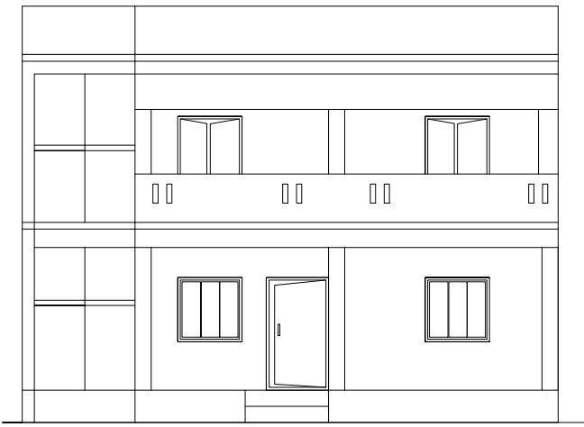
FRONT ELEVATION
