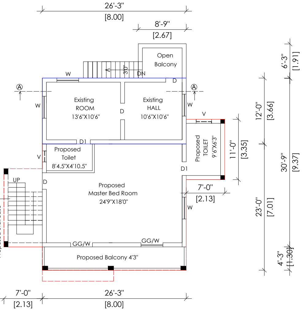
EXISTING FIRST FLOOR AND PROPOSED ADDITIONAL CONSTRUCTION FIRST FLOOR PLAN
