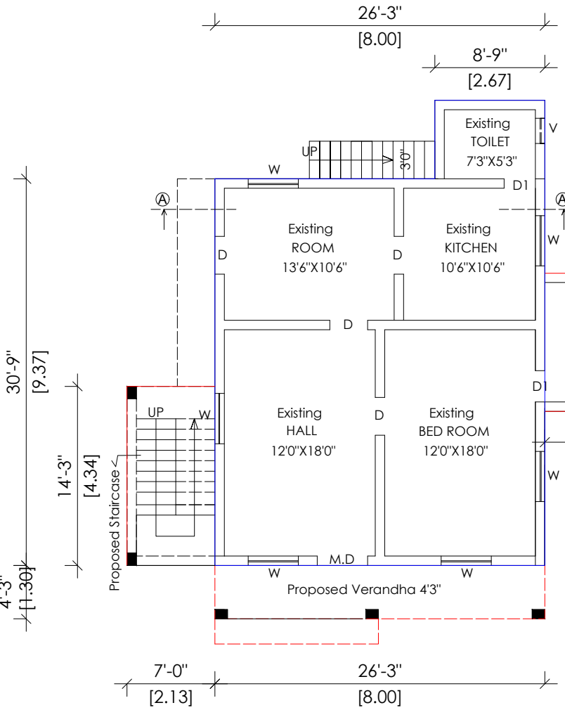
EXISTING GROUND FLOOR AND PROPOSED ADDITIONAL CONSTRUCTION GROUND FLOOR PLAN
