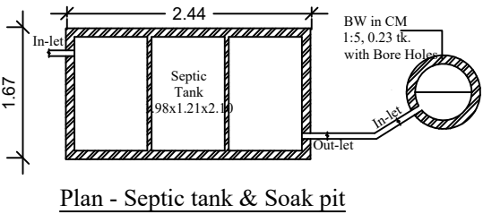
Plan - Septic tank & Soak pit
