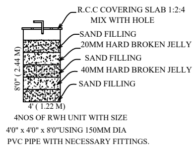
RAIN WATER HARVEST UNIT
