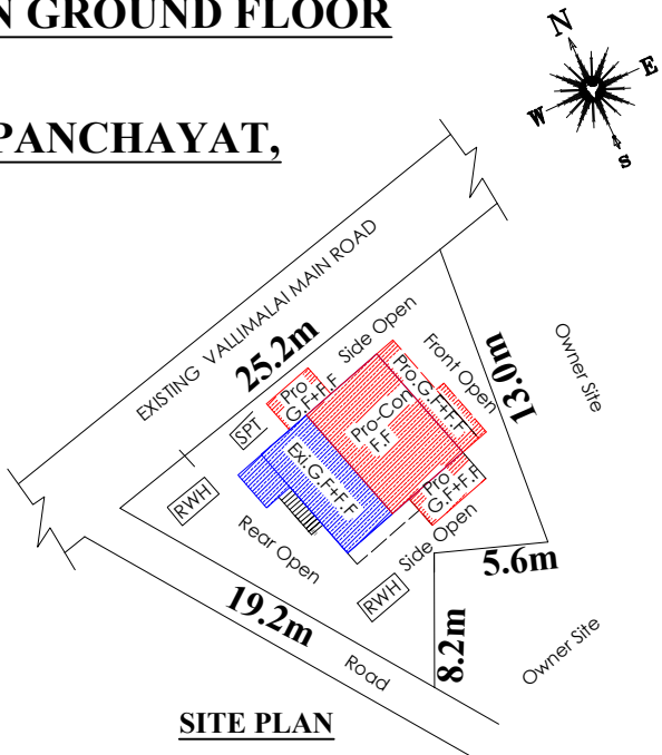
SITE PLAN
