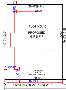
SCALE- 1:100
