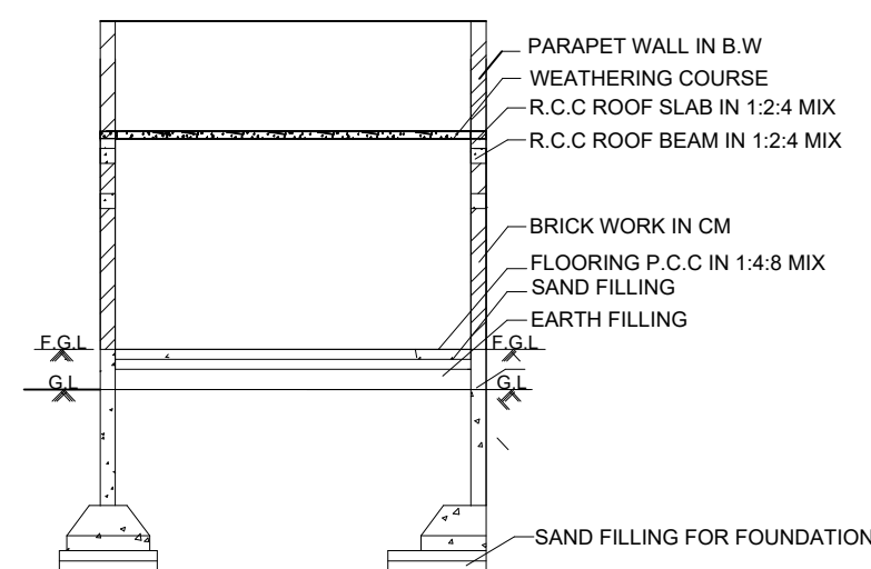
SECTION ON-AA
