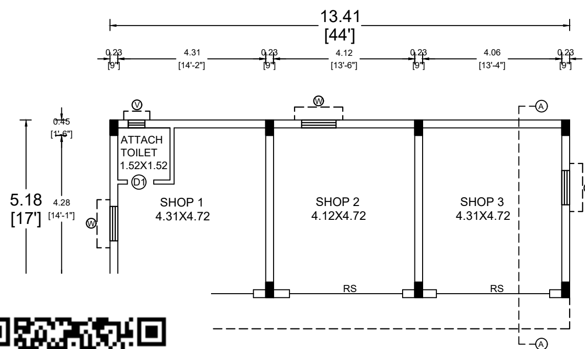
SED GROUND FLOOR PLAN
