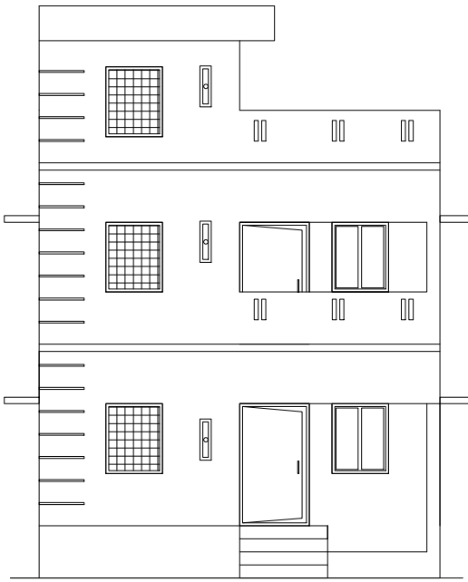
FRONT ELEVATION
