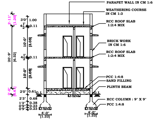
SECTION - KK
