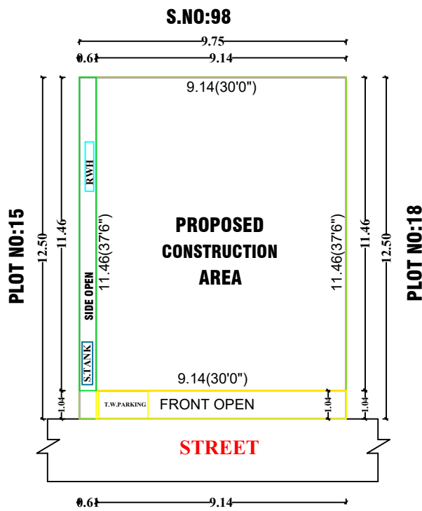
SITE PLAN SCALE : 1:100 SURVEY NO:102/1A1A1A1 PLOT NO-16 & 17 MINI GOLDEN NAGAR THALAYATHAM VILLAGE & PANCHAYAT GUDIYATHAM TALUK VELLORE DISTRICT
