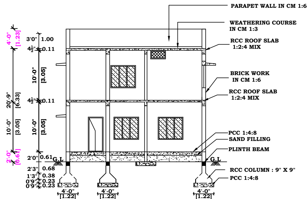
SECTION - KK
