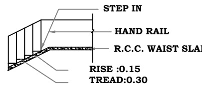
STAIR DETAILS
