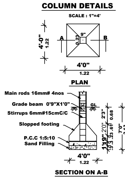
COLUMN DETAILS
