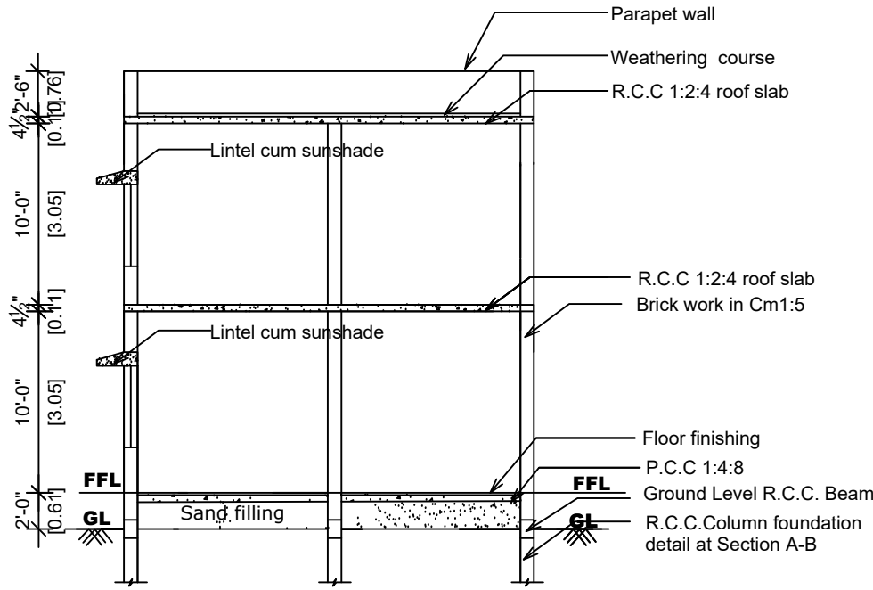
SECTION ON 'RK'
