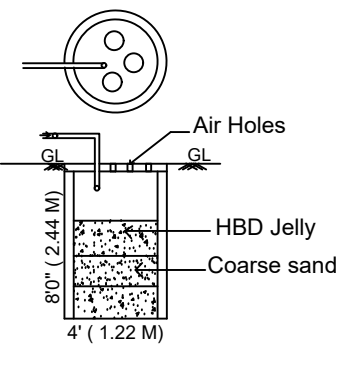
RAIN WATER HARVESTING TANK DETAIL
