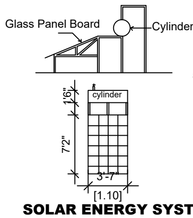
SOLAR ENERGY SYSTEM
