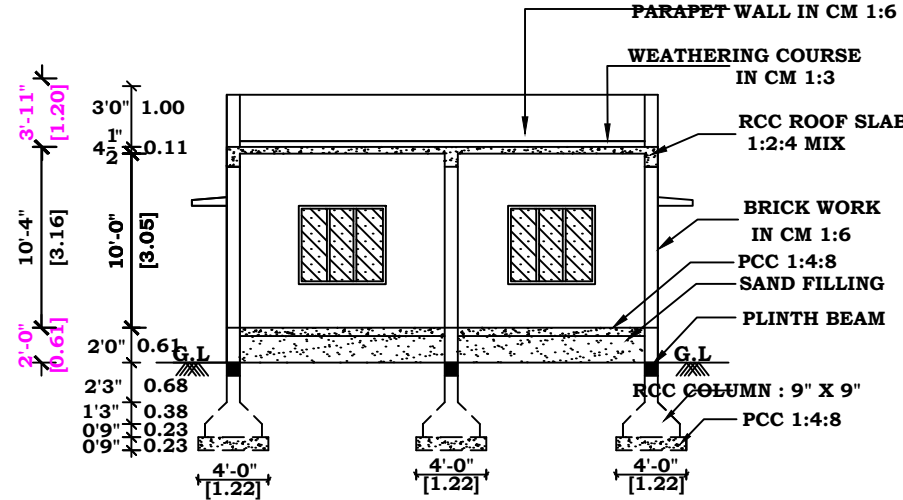
SECTION - KK
