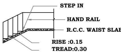
STAIR DETAILS
