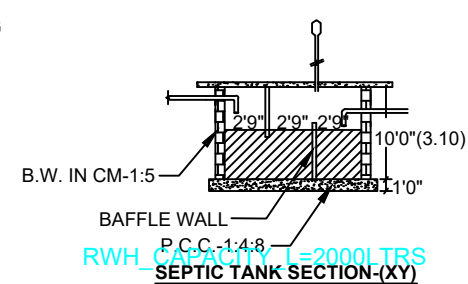
RWH_CAPACITY=2000LTRS SEPTIC TANK SECTION-(XY)
