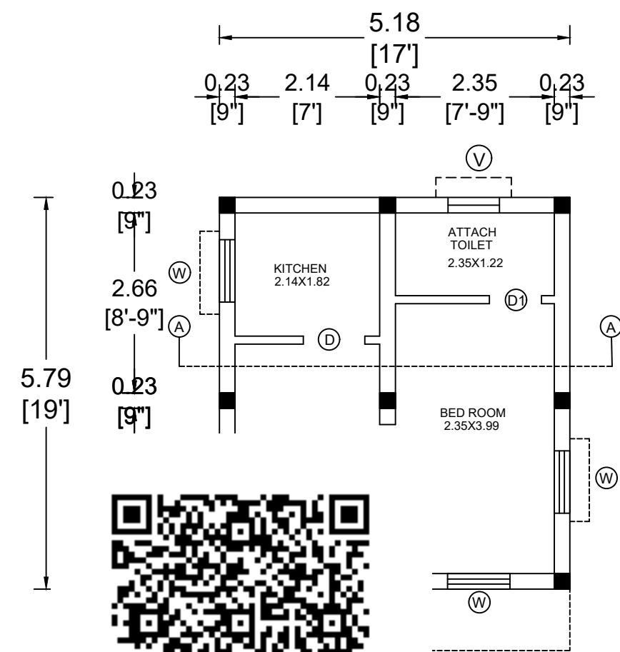
FLOOR PLAN
