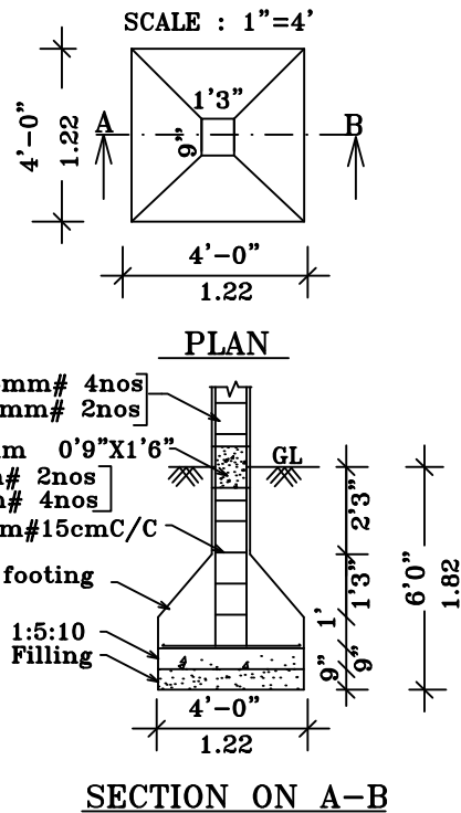
COLUMN DETAILS
