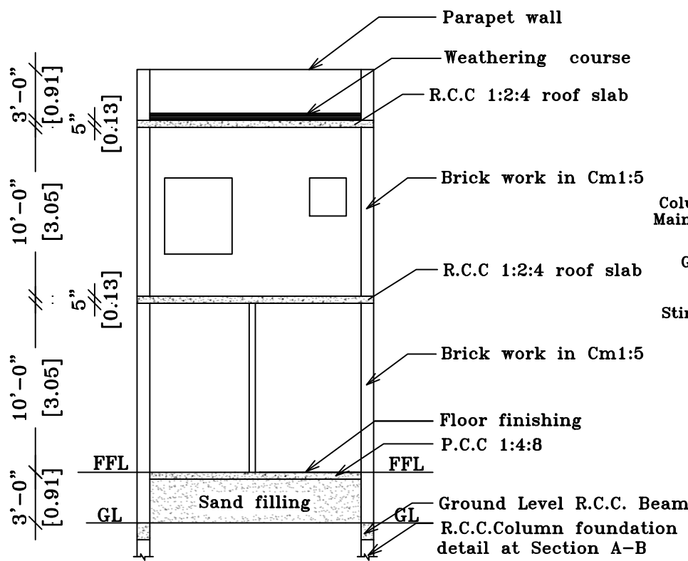
SECTION ON 'SA'
