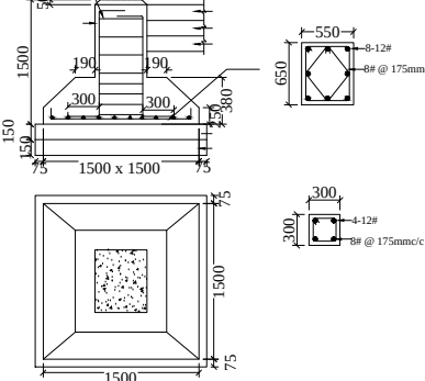
Foundation Details
