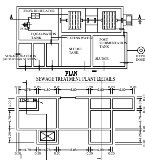
Sewage Treatment Plant Details
