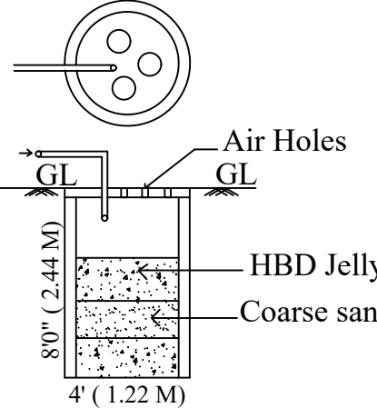
RAIN WATER HARVESTING TANK DETAIL
