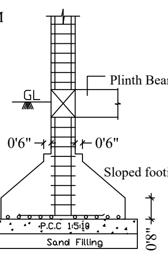
SECTION ON JS1
