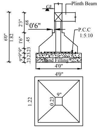
COLUMN DETAIL NOT TO SCALE
