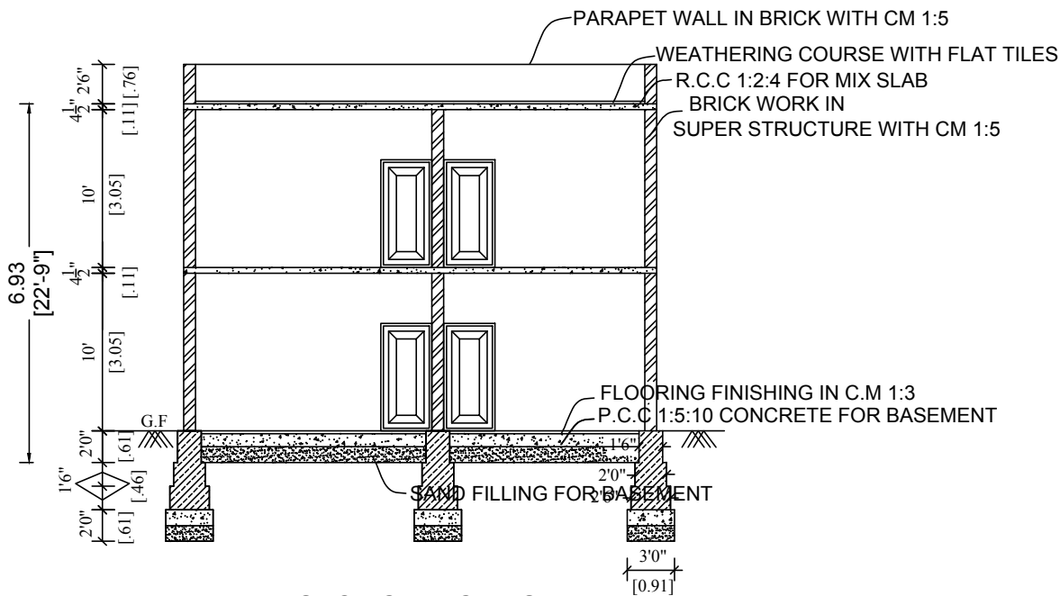
SECTION NO R-S
