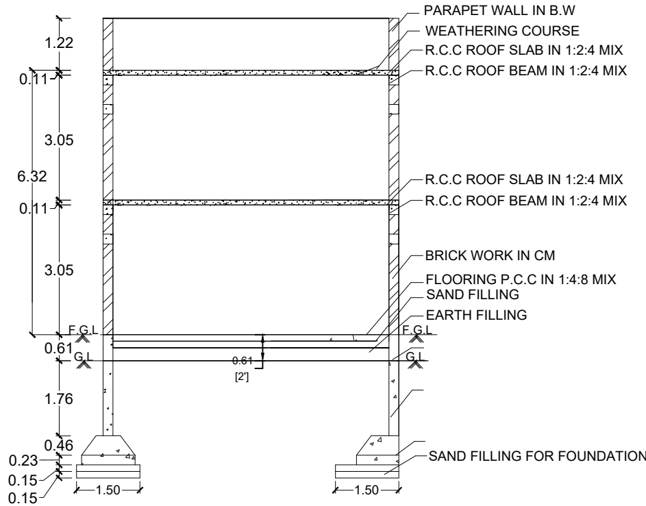
SECTION ON-AA
