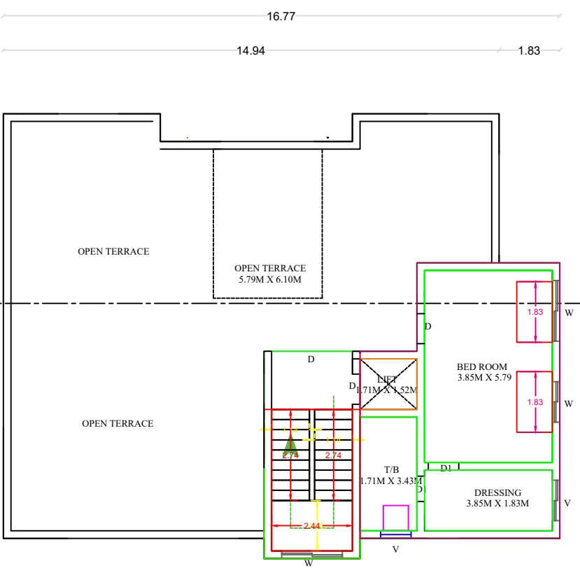
PRO.SECOND FLOOR PLAN
