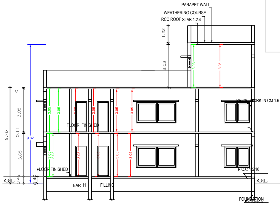
SECTION "A-B"
