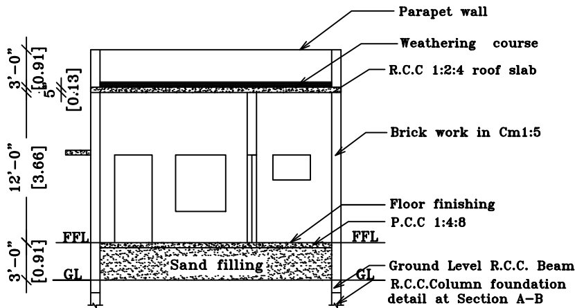
SECTION ON 'SA'
