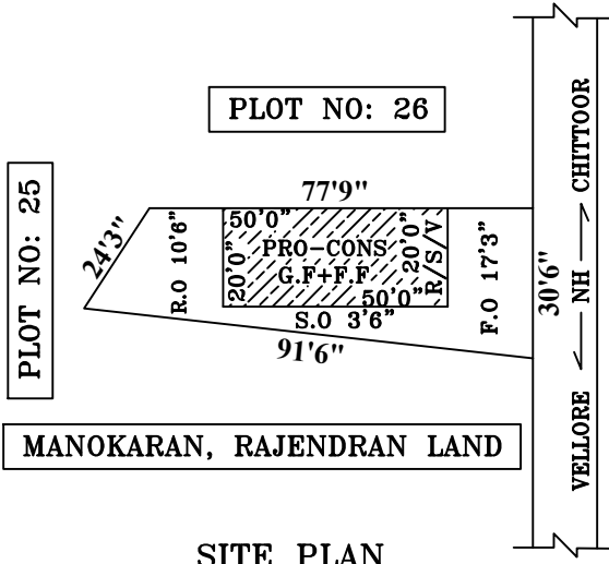
SITE PLAN
