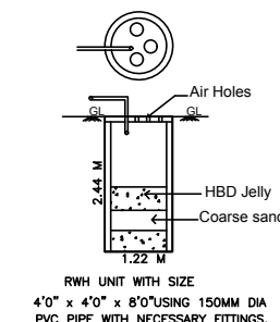
RAIN WATER HARVESTING TANK DETAIL
