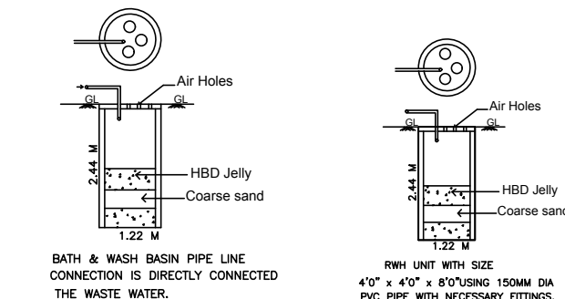
WASTE WATER RECYLING TANK DETAIL
