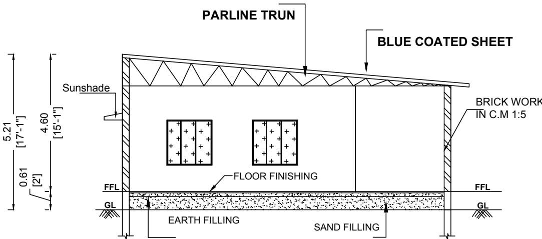
SECTION ON "JS"
