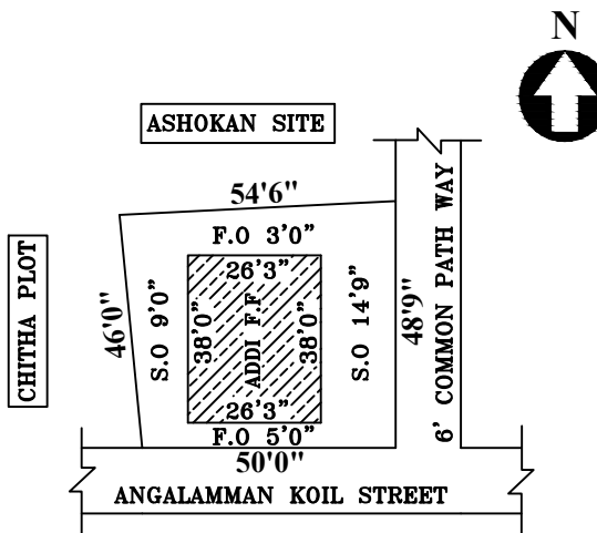
SITE PLAN
