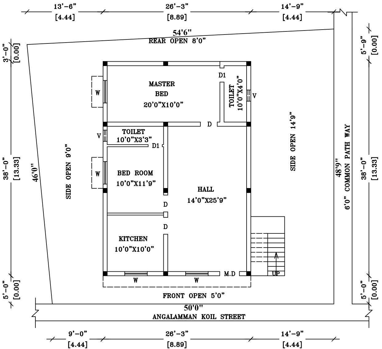
EXI. GROUND FLOOR PLAN
