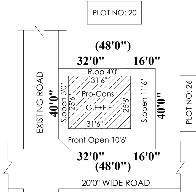
SITE PLAN SCALE:1INCH = 33FEET
