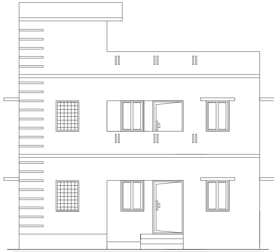
FRONT ELEVATION
