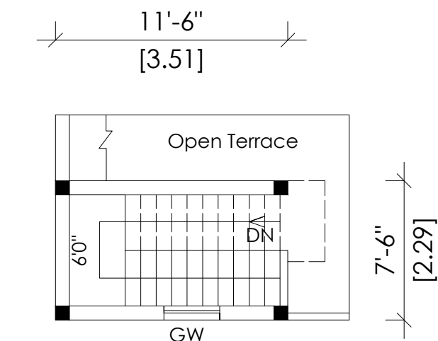
HEAD ROOM PLAN
