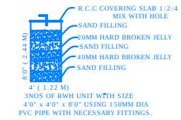
Rain Water Harvesting unit
