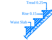
Section of the Staircase Not to scale
