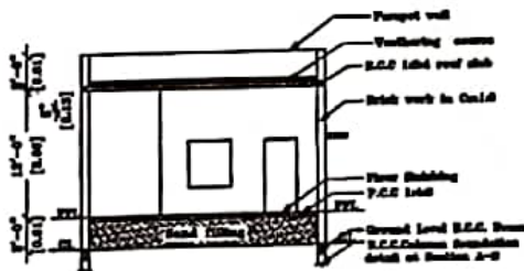
SECTION ON 'SA'
