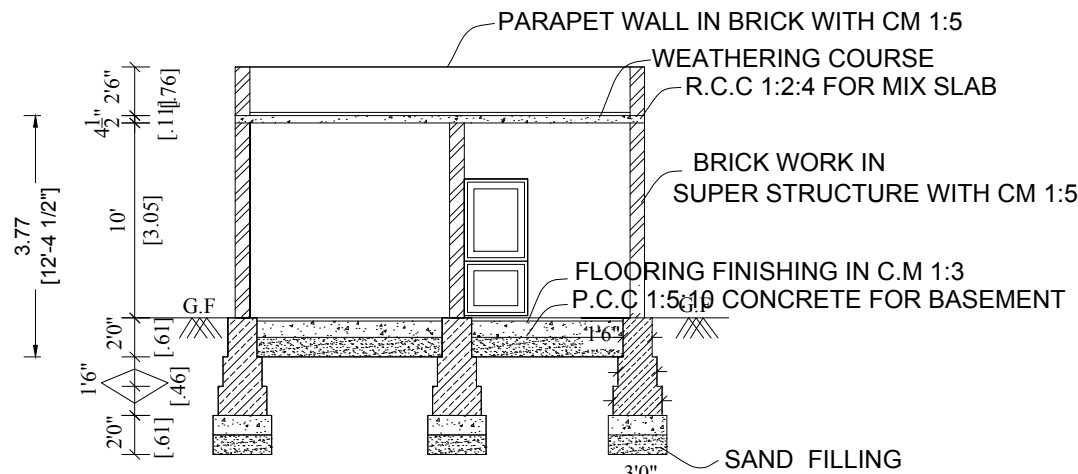
SECTION ON - R S
