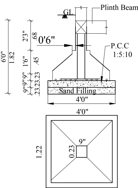
COLUMN DETAIL NOT TO SCALE
