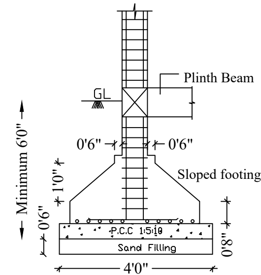
ISOLATED FOOTING / COLUMN DETAIL
