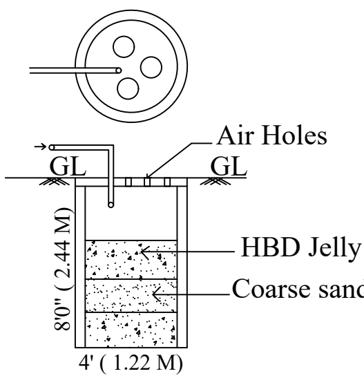
RAIN WATER HARVESTING TANK DETAIL
