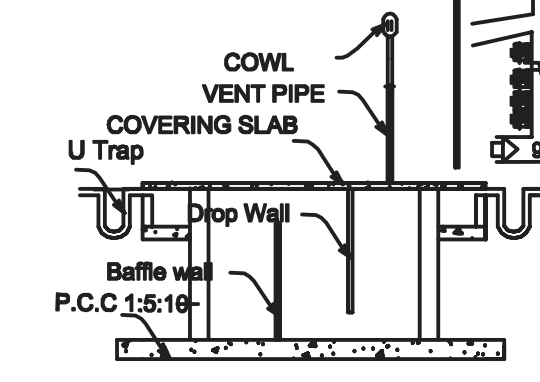
SECTION ON JS1
