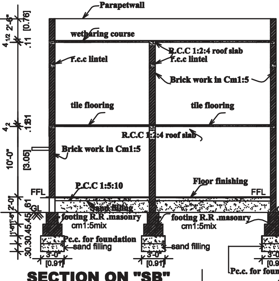
SECTION ON "SB"
