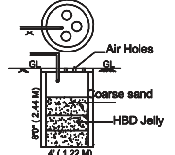
RAIN WATER HARVESTING TANK DETAIL
