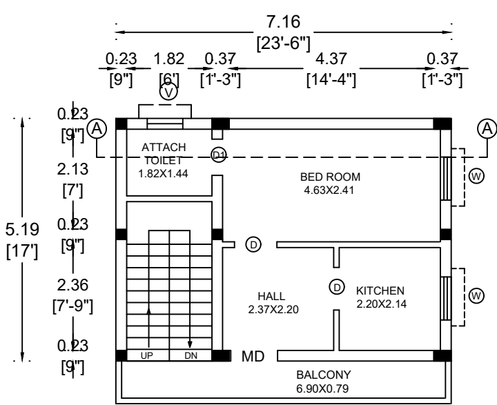
FIRST FLOOR PLAN (RESIDENTIAL BUILDING)
