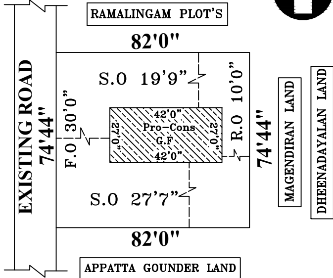
SITE PLAN
