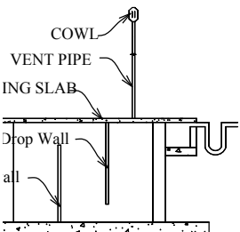
SECTION ON JS1
