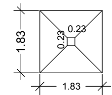
FOOTING
