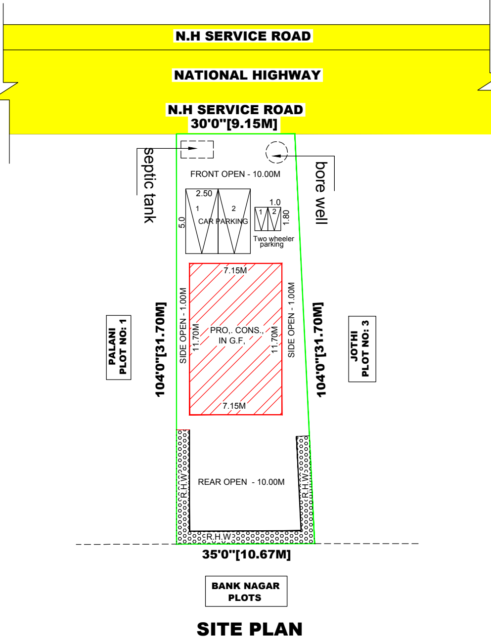
SITE PLAN
