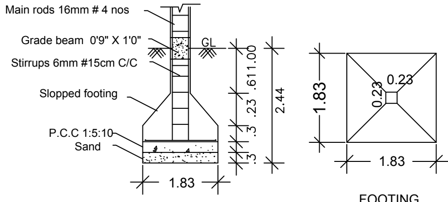
ISOLATED FOOTING
