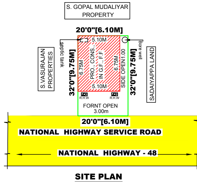
SITE PLAN
