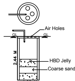
RAIN WATER HARVESTING TANK DETAIL
