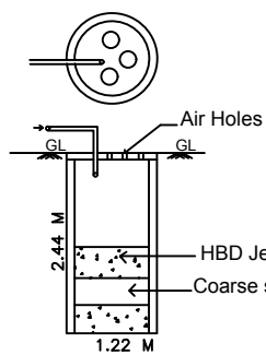
WASTE WATER RECYLING TANK DETAIL
