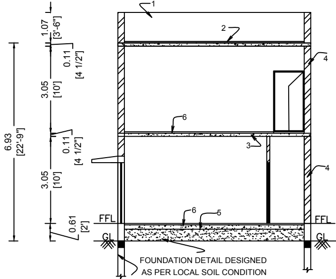
SECTION ON "JS"
