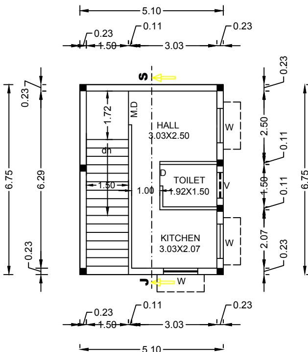
PRO., FIRST FLOOR PLAN (RESIDENTIAL)
