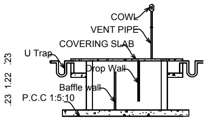
SECTION ON JS1 in inlet, outlet & Vent pipe will be covered with net in inner side and top of vent pipe.
